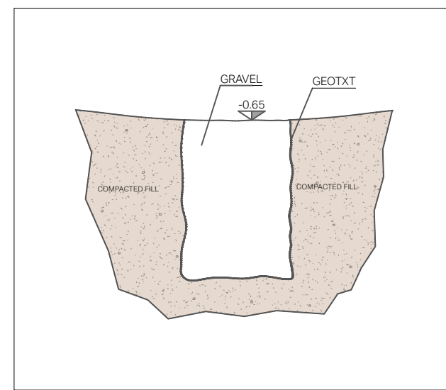
TYP. DETAIL - FRENCH DRAIN
