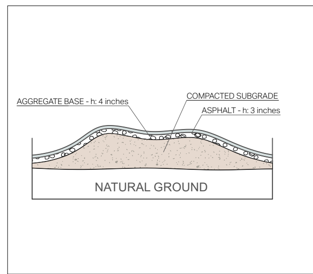
TYP. DETAIL - MATERIALS
