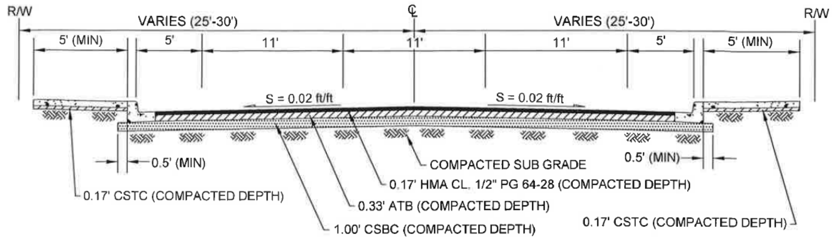
TYPICAL SECTION
