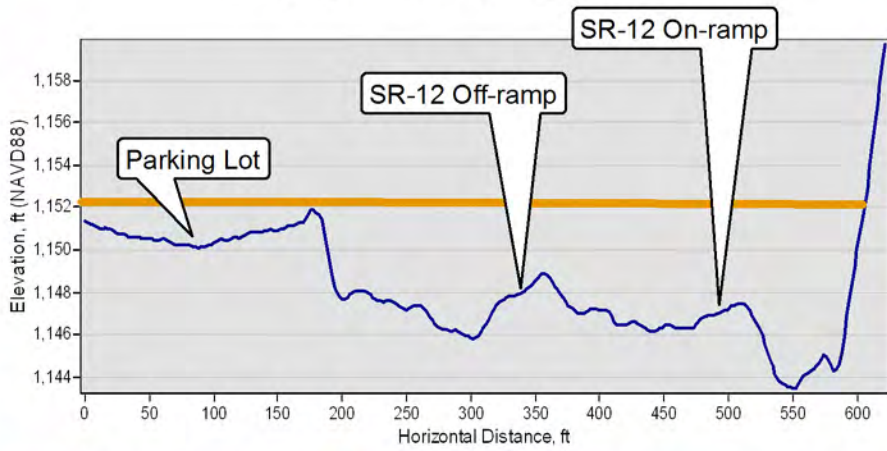
Emergency berm profile (looking northwest)
